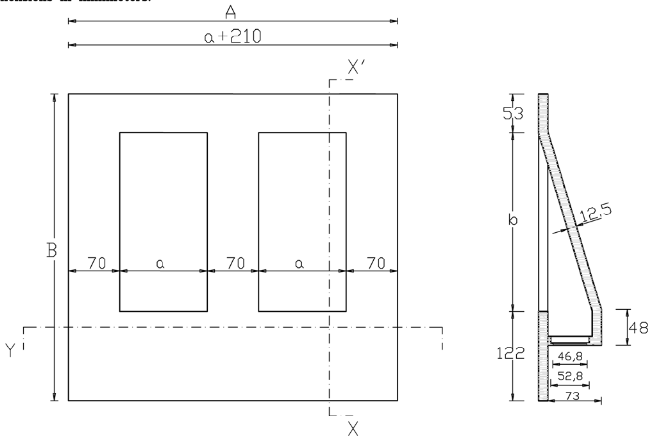
FRONT VIEW
