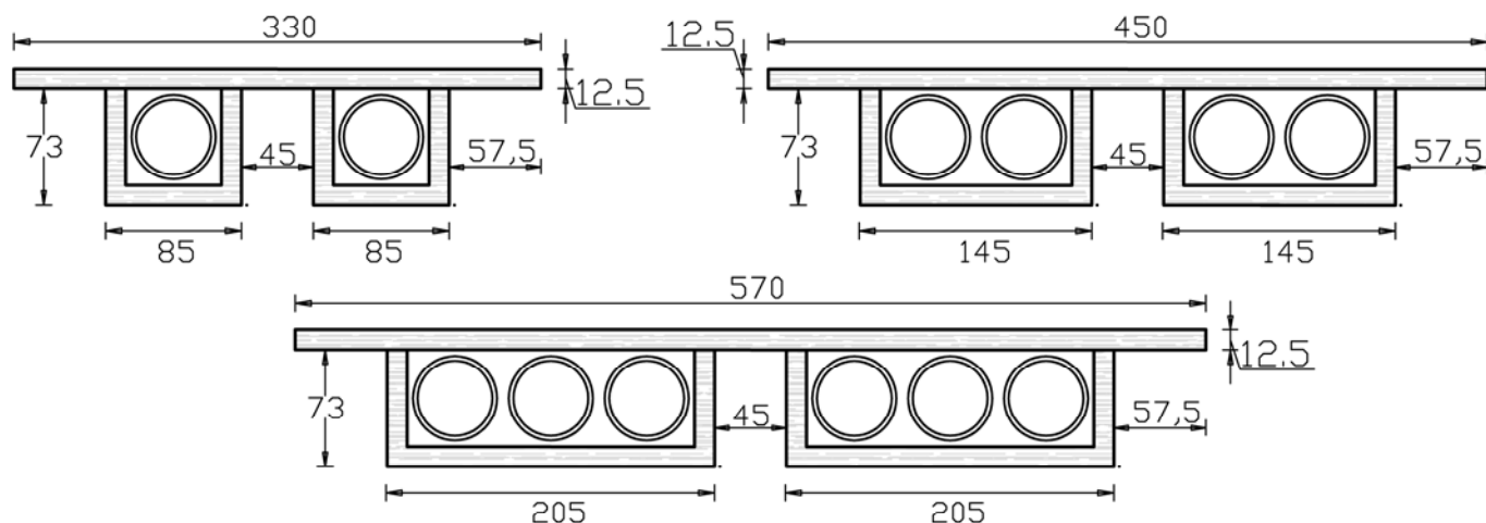
SECTION Y-Y'
